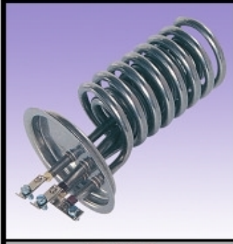
YIL1085 IHLAS TİPİ ŞOFBEN ISITICI 220 V. 3000+4500 W. (6.5Ø- Cr-ni)
