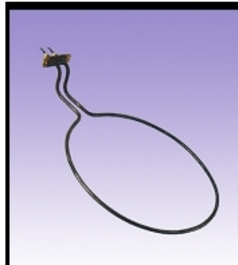
YIL1125 220 V. 750 W. (Ø 6.5 mm.CrNi)
