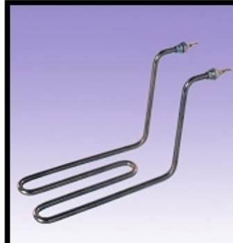
230 V. 2500 W. (8.5Ø- Cr-ni)
