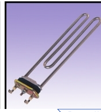
220 V. 1950 W. (8.5 \phi - Cr-ni)
