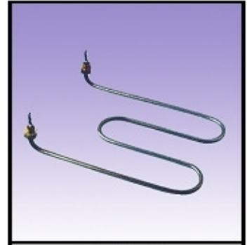
YIL1078 M TİPİ KIVRIK SEMAVER REZ. 220 V. 2000 W. (8.5 \phi - Cr-ni)
