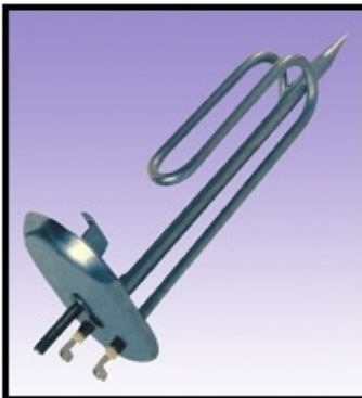
YIL1244 1950 W. 220 V. (8.5Ø-Cr-ni)
