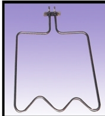
YIL1117 230 V. 1000 W. (Ø 6.5-8.5 mm.CrNi)
