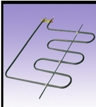
YIL1124 220 V. 2000 W. (Ø 6.5 mm.CrNi)
